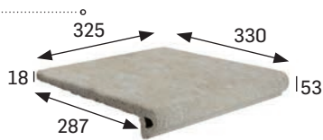
PELDAÑO REDONDEADO 33 ROUNDED STAIR-TREAD 33 [330x330x18 mm]
