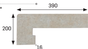
ZANQUÍN IZDA. RECTO STRAIGHT STRING LEFT SIDE * [390x80/200x100x16 mm]
