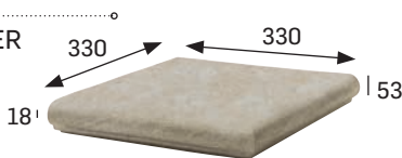
RODAPIÉ SKIRTING BOARD [325x80x16 mm]
