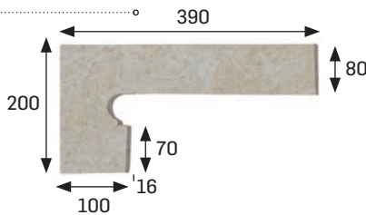
ZANQUÍN DCHA. STRING RIGHT SIDE [390x80/200x100x16 mm]
