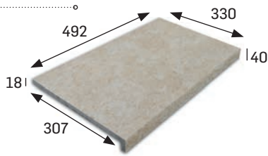
PELDAÑO RECTO 50 STRAIGHT STAIR-TREAD 50 [492x330x18 mm]
